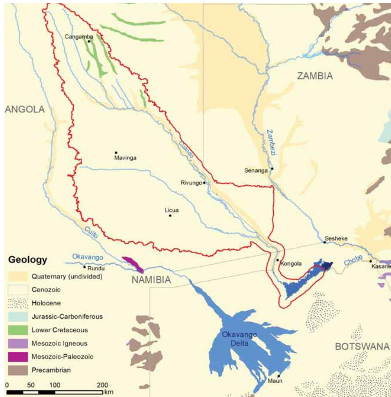
Figure 33: Geological features of the Cuando River Basin.
