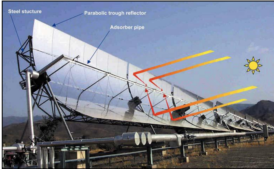
Elements of a Parabolic Trough System
