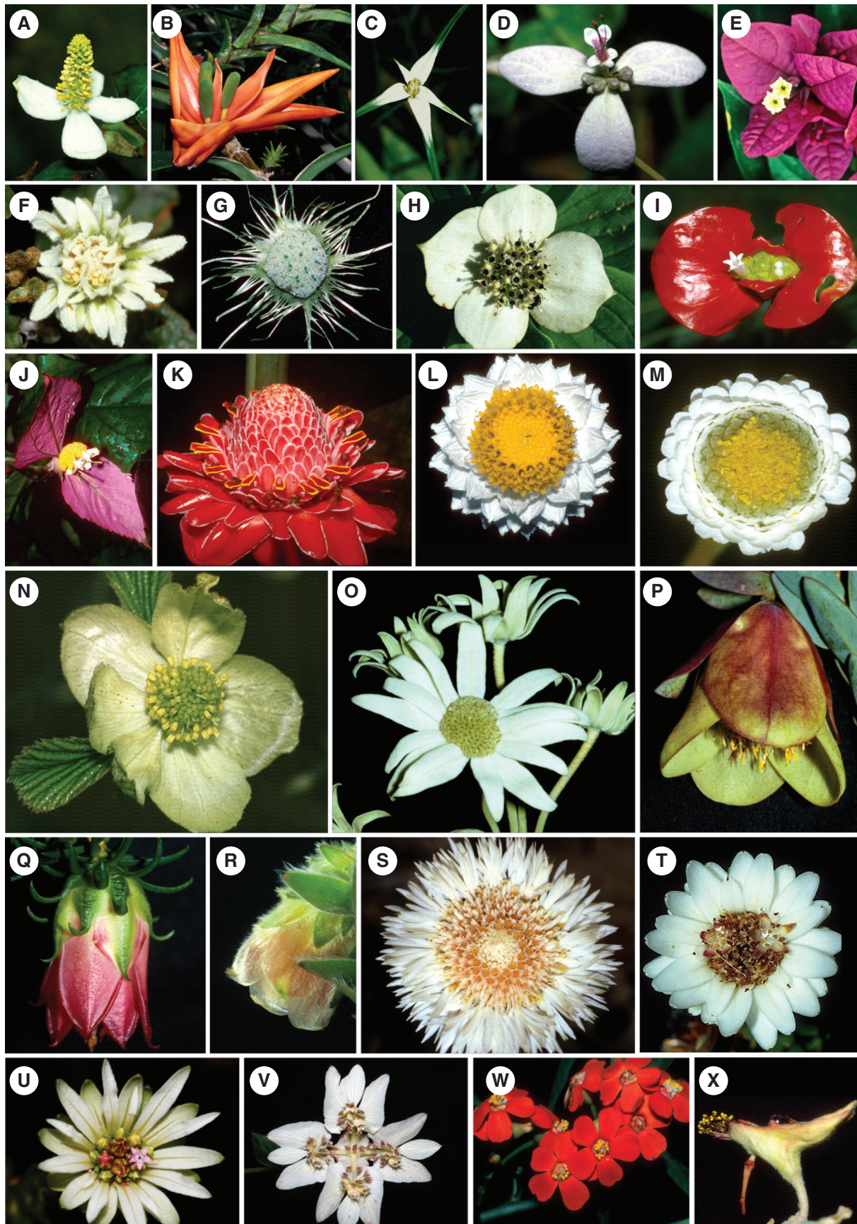
FIG. 5. Pseudanthia sensu stricto with showy extrafloral elements. (A) Spike with showy bracts: Houttuynia cordata (Saururaceae). (B) Three spadices with showy bracts: Freycinetia sp. (Pandanaaceae). (C) Cluster of spikelets with showy bracts: Dichromena ciliata (Cyperaceae). (D) Cyme with showy bracts: Congea velutina (Lamiaceae). (E) Three-flowered unit: Bougainvillea glabra (Nyctaginaceae). (F) Cymoid with showy bracts: Lasioptelum discolor (Malvaceae). (G) Cymoid-like head with showy bracts: Dorstenia yambuyaensis (Moraceae). (H, I) Thyrses with showy bracts: (H) Cornus canadensis (Cornaceae); (I)
