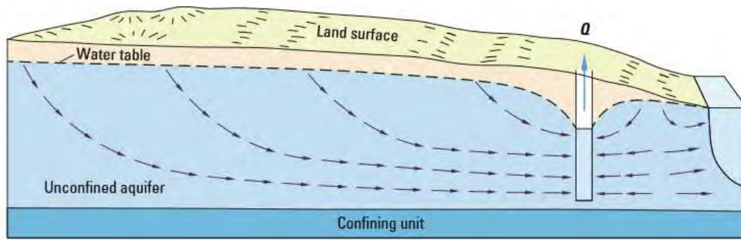
FIGURE 2.4: EFFECTS OF PUMPING ON DISCHARGES TO A STREAM. AS THE CONE OF DEPRESSION EXPANDS OUTWARD FROM THE WELL, THE WELL BEGINS TO CAPTURE GROUNDWATER THAT WOULD OTHERWISE HAVE DISCHARGED TO THE STREAM (SOURCE: BARLOW AND LEAK (2012))
