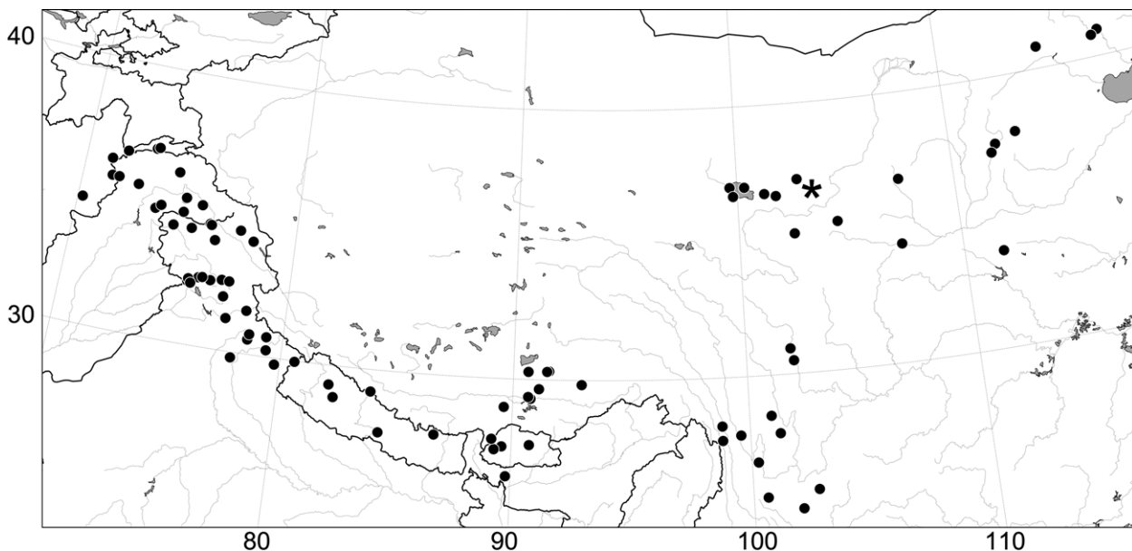
Fig. 7. Distribution of Dysphania nepalensis based on the specimens seen (dots). Location of the holotype specimen of Dysphania kitiaae (asterisk).
