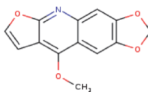
Maculine (17)
