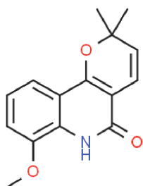
8-methoxyflindersine (12)
