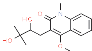
Flindersiamine (16)
