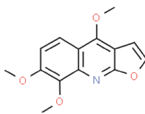
Skimmianine (15)
