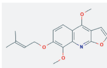
haplopine-3,3-dimethylallylether (9)
