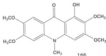
Arborinine (13)
