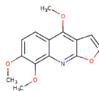
isohaplopine-3,3-dimethylallylether (7),
