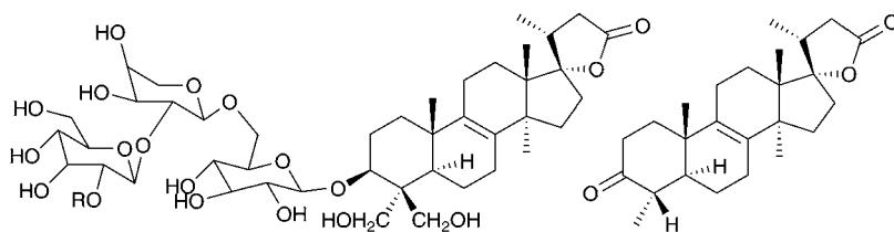
25 R = β-apiofuranosyl
