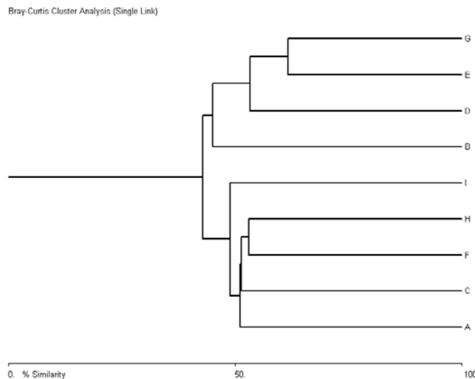
Figure 3. 4 Cluster analysis for the nine sectors surveyed using plot data
