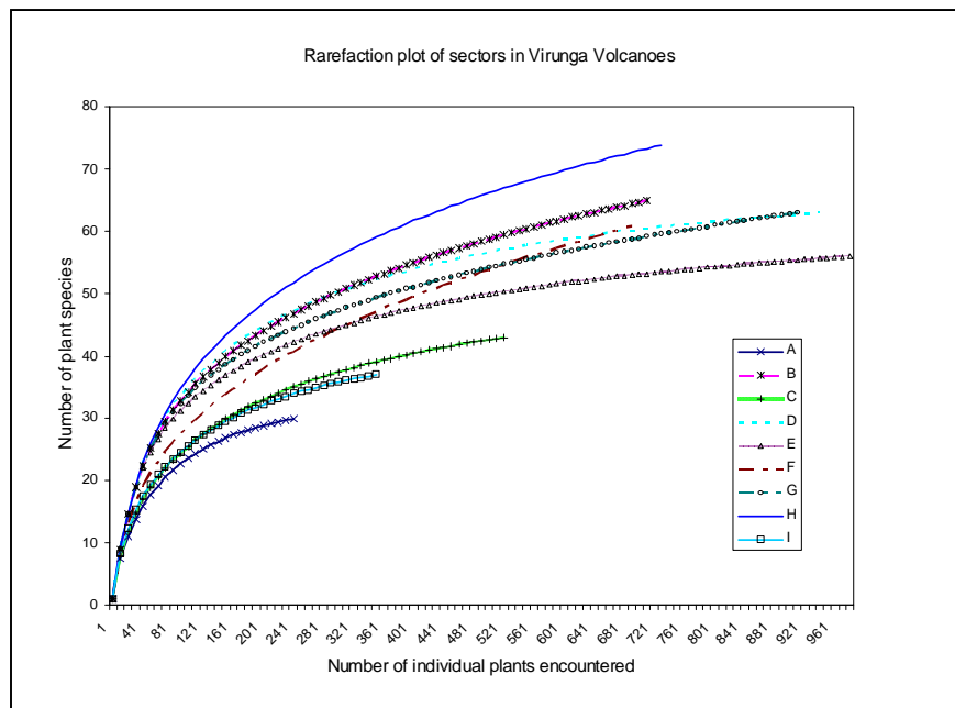
Figure 3. 3 Plant species richness in sectors.
