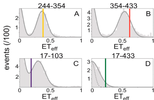
Figure 8. Effect of charge screening on the transfer efficiencies of tau protein labeled with FRET dyes at different positions within the chain. Transfer efficiency ( ET_{\text{eff}} ) histograms in 500 mM NaCl are shown for the intramolecular pairs 244–354 (A), 354–433 (B), 17–103 (C), and 17–433 (D), with colored vertical lines indicating the peak position for each construct at 50 mM NaCl. Note that the constructs respond to charge screening very differently, in some cases leading to expansion and in others to collapse. Reprinted with permission from ref 151. Copyright 2012 American Chemical Society.
