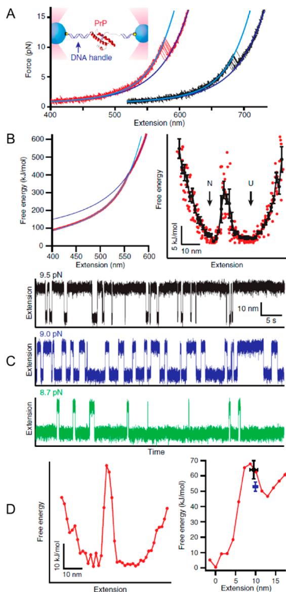
Figure 21. Characterization of the PrP unfolding energy landscape via passive force clamp OT experiments, as described in Yu et al. 317 (A) Unfolding (red) and refolding (black) force–extension curves obtained by ramping up the force applied on a PrP-containing DNA–protein construct (inset) prepared as described by Ceconi et al. 265,327 Continue lines are WLC fits of the folded and unfolded states. Abrupt contour length changes are observed at a force of \sim 9 pN, corresponding to folding and unfolding transitions (here occurring in a two-state process). (B) (Left) Free energy profile at zero force reconstructed from the force–extension traces exemplified in A via the Hummer–Szabo method, 226,276 mostly determined by the elastic behavior of the DNA handles. (Right) PrP energy landscape under an applied force of 9.1 pN displayed as the average (black line) of different sets of force–extension curves (red dots). (C) Extension vs time plots recorded at different constant forces, showing a clear two-state folding–unfolding behavior. The force F_{1/2} at which the two folding states were observed to be identically populated was again \sim 9 pN. (D) (Left) Unfolding free energy profile at F_{1/2} after deconvolution. (Right) Same energy landscape “tilted” to 0 pN applied force. The position and height of the energy barrier is shown to be in excellent agreement with the values (black, unfolding; blue, refolding) found via kinetic analysis of force–extension curves exemplified in A and B. Adapted with permission from ref 317. Copyright 2009 National Academy of Sciences.
