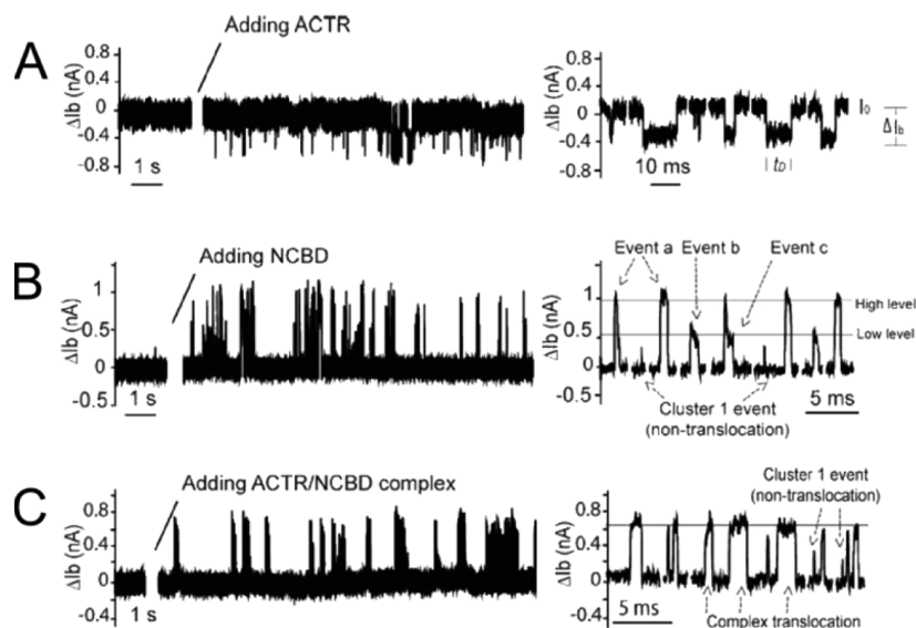
Figure 25. Translocation traces of (A) ACTR, (B) NCBD, and (C) the ACTR+NCBD complex through a solid-state nanopore in a silicon nitride membrane at an applied voltage of 300 mV as described in Japrung et al. 358 Both IDPs are observed to translocate establishing a variety of different interactions with the nanopore, while their structured complex only shows one type of event. Interestingly, both NCBD and the ACTR+NCBD complex show current enhancement during interaction with the pore, while ACTR induces resistive pulses. Reprinted with permission from ref 358. Copyright 2013 American Chemical Society.
