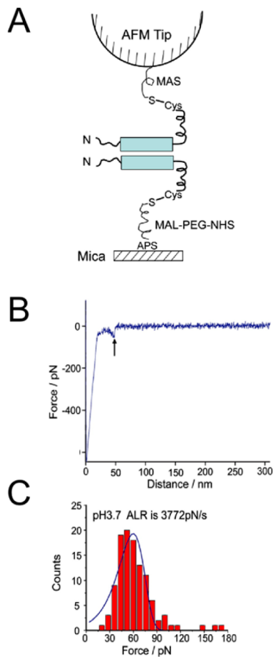
Figure 17. \alpha Syn intermolecular interactions probed via AFM-based SMFS as reported by Yu et al. 295 (A) Schematization of the experimental setup: \alpha Syn molecules are covalently anchored via silane chemistry to the AFM probe and a mica surface in a reciprocal orientation that should enhance contacts between the respective amyloidogenic N-terminal regions (gray boxes). (B) Force curve representative of those considered to contain the mechanical rupture signature of a bimolecular \alpha Syn interaction at pH 3.7. (C) Rupture force distribution for the mechanical events exemplified in B. The continuous line is the fit of the experimental data collected at pH 3.7 with the probability density function (PDF). The maximum of the PDF was found to be at 61.6 \pm 2.3 pN. Reprinted with permission from ref 295. Copyright 2008 Elsevier.
