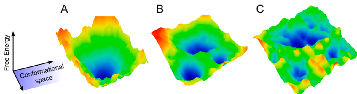
Figure 2. Pictorial representation of the free energy landscapes of proteins with an increasing degree of intrinsic disorder. Free energy landscapes of structured proteins characterized by a stable three-dimensional structure are dominated by a single deep funnel (A), while those corresponding to proteins able to adopt a limited number of structures show a small number of basins of similar depth separated by substantial barriers (B). Disordered proteins are instead characterized by shallow energy landscapes (C) with several local minima of comparable free energy, separated by low barriers allowing fast interconversion kinetics between conformations.
