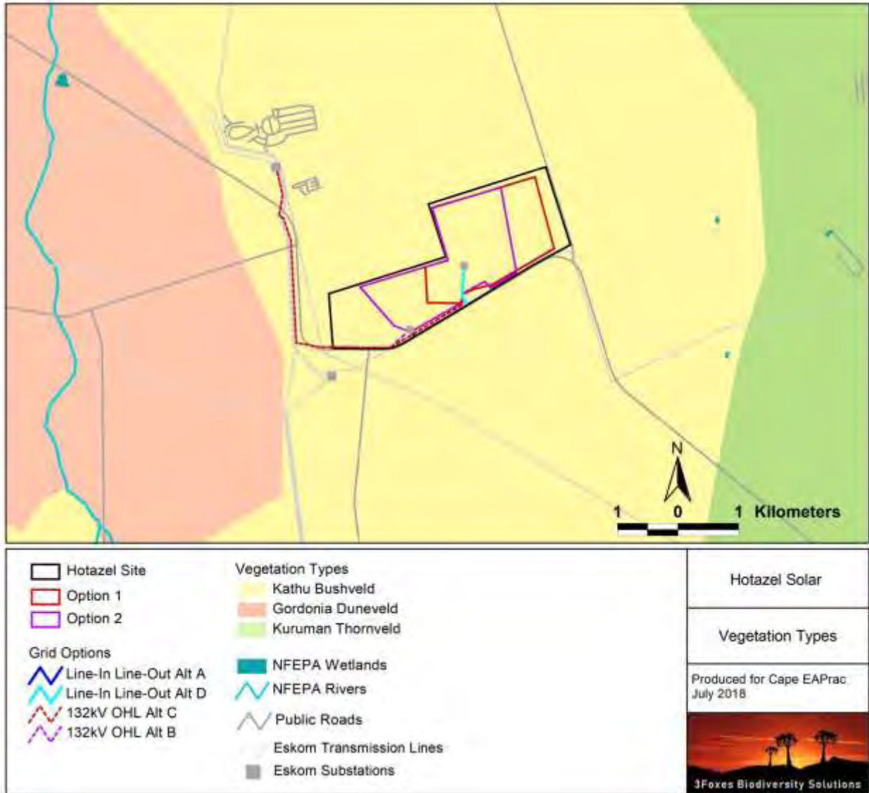
Figure 2. Broad-scale overview of the vegetation in and around the Hotazel site. The vegetation map is an extract of the national vegetation map as produced by Mucina and Rutherford (2006/2012), and also includes wetlands delineated by the NFEPA assessment (Nel et al. 2011).
